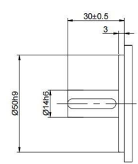
(400W)60mm Servo
