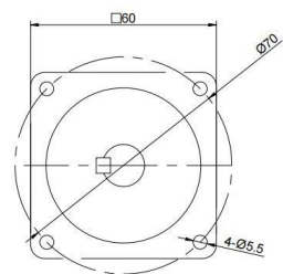
(400W)60mm Servo
